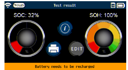
Battery needs to be recharged (Unsatisfactory SOC, good SOH).
