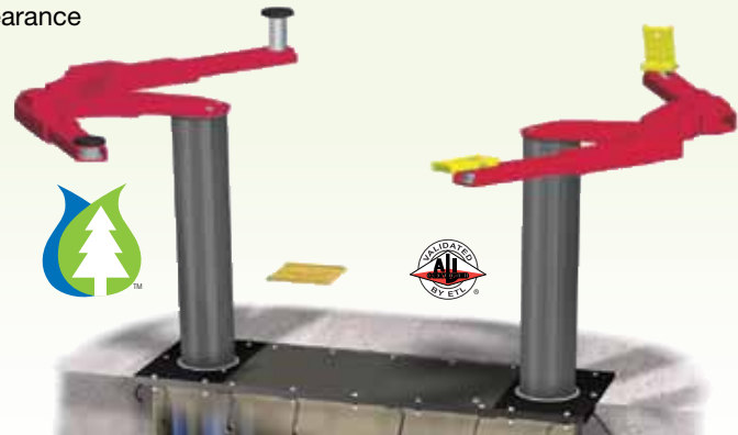
Shown: ROTSL210RA on left / ROTSL210 on right. Must choose preference when ordering. Shown with optional adapter extensions. TRIO arms only available on 10,000 lbs. capacity models.
